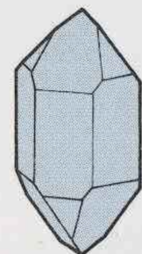
TRIGONAL/ HEXAGONAL
