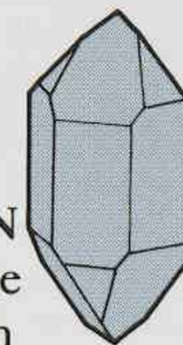
TRIGONAL/ HEXAGONAL
