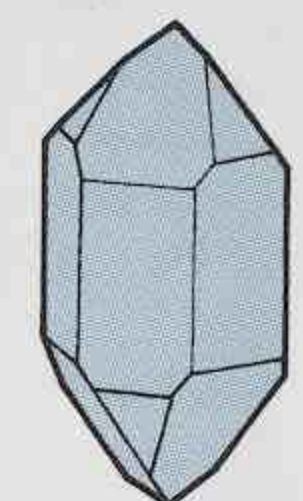
TRIGONAL/ HEXAGONAL
