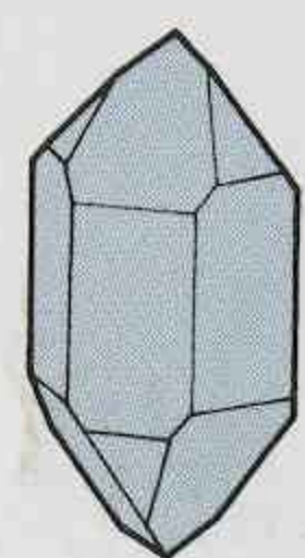
TRIGONAL/ HEXAGONAL
