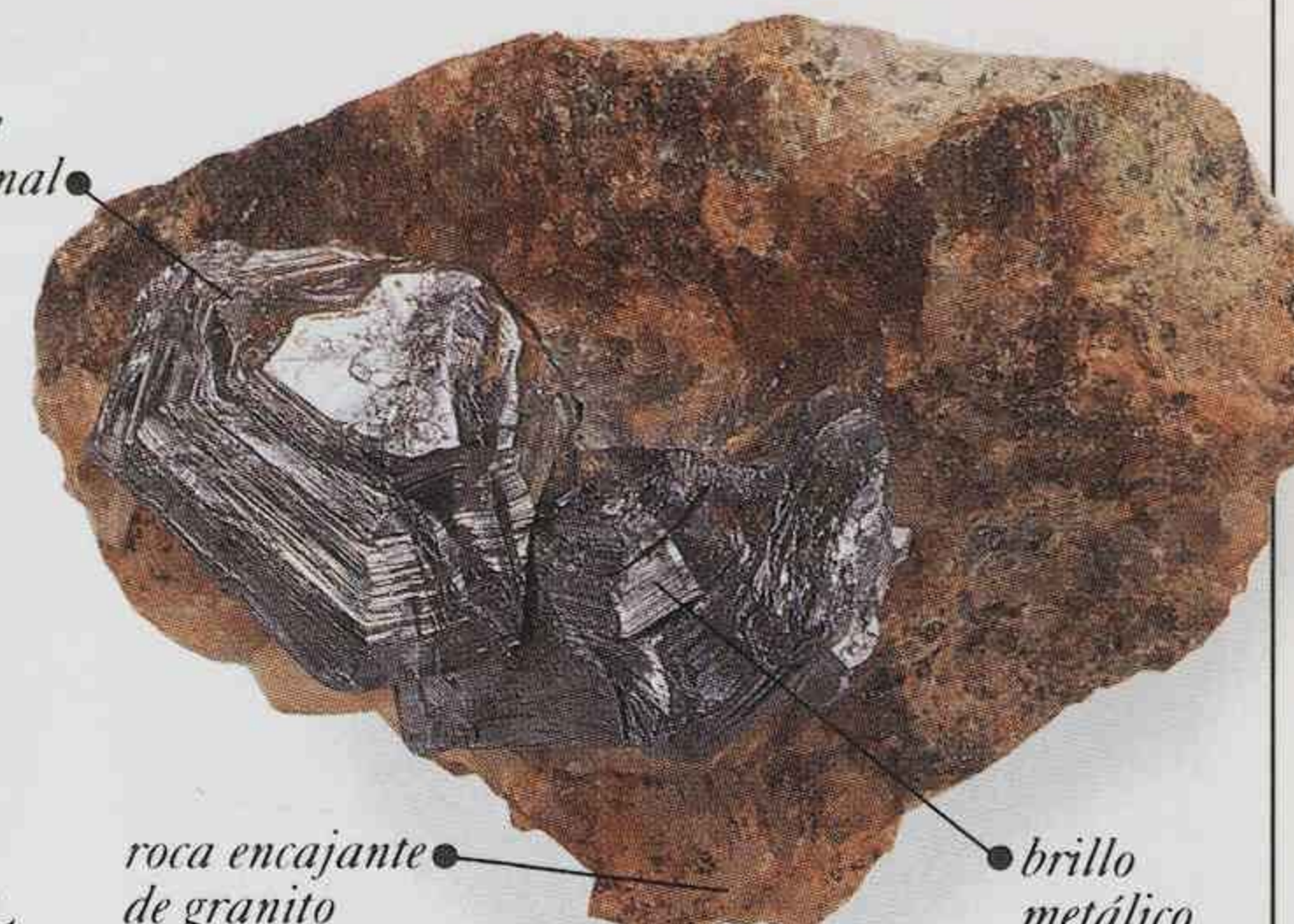
TRIGONAL/ HEXAGONAL
