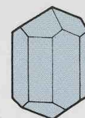
TETRAGONAL
