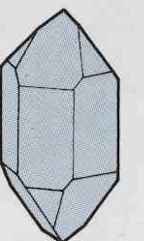
TRIGONAL/ HEXAGONAL
