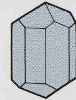
TETRAGONAL
