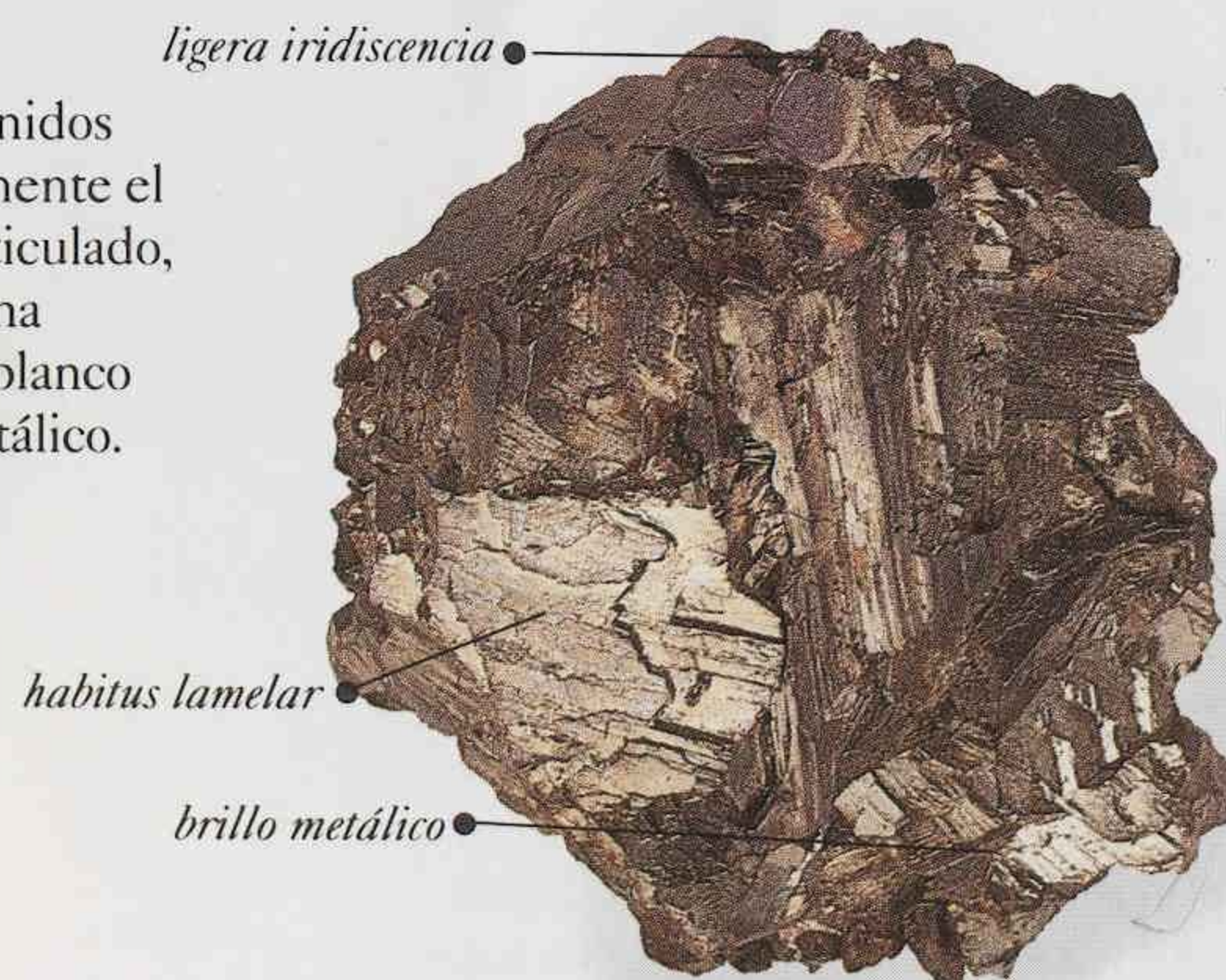
TRIGONAL/ HEXAGONAL
