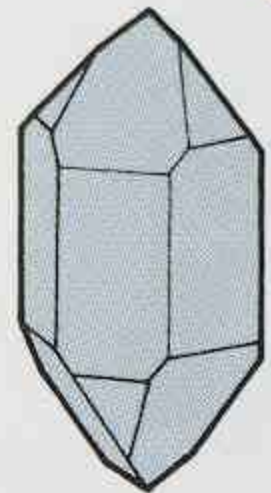
TRIGONAL/ HEXAGONAL
