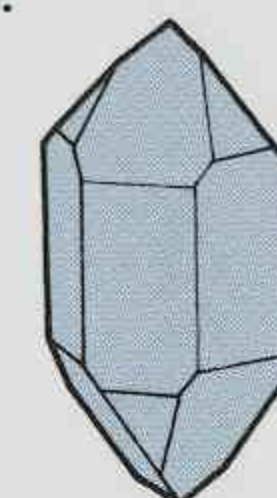
TRIGONAL/ HEXAGONAL
